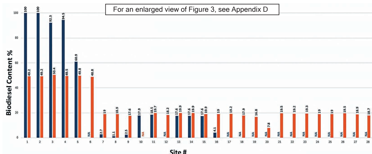
Figure 3. Biodiesel content change between Visits 1 and 2, showing the sites reaching the desired biodiesel levels.
