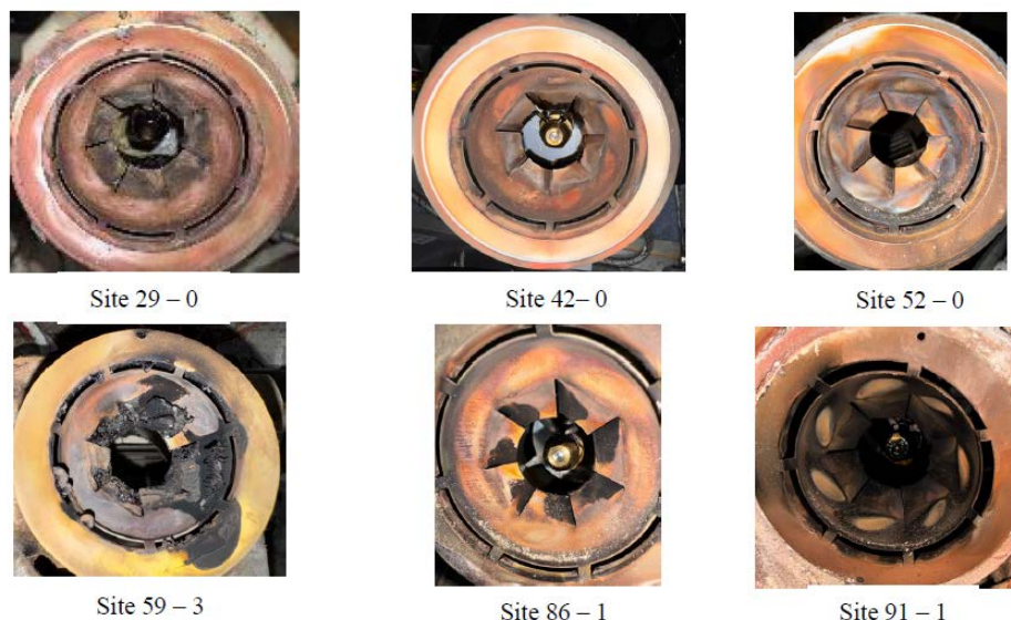
Figure 8. Photos of the retention heads from Level 2 sites with furnaces during visit period 5. The number after the dash indicates the coking level score.
