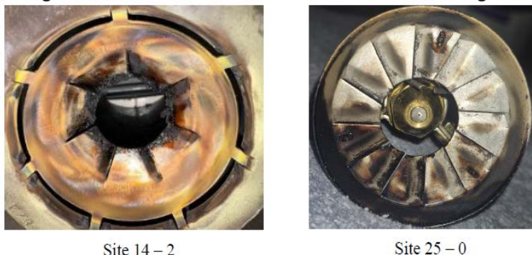
Figure 9. Photos of the retention heads from sites with water heaters during Visit 5. The number after the dash indicates the coking level score.
