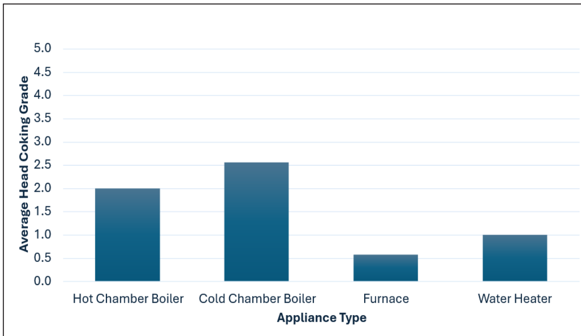
Figure 10. Average head coking grades for each appliance type from Visit 5.
