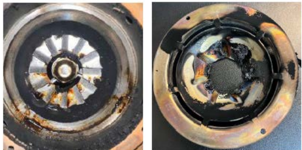
Figure B-3. Examples of retention heads with a rating of 2
