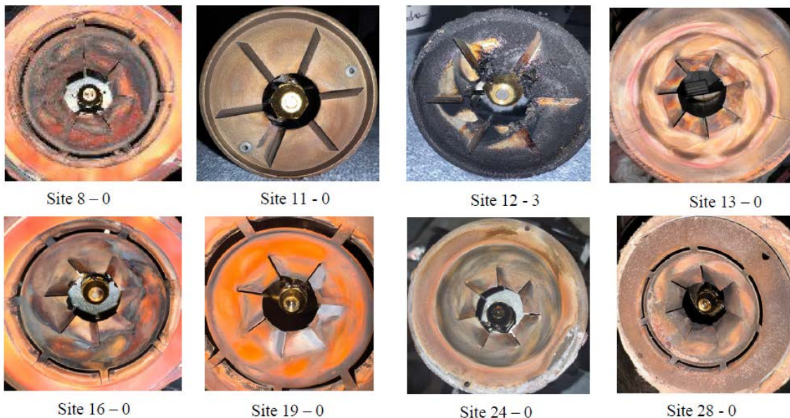
Figure 7. Photos of the retention heads from Level 1 sites with furnaces during visit period 5. The number after the dash indicates the coking level score.
